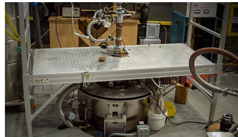
17 Tesla Superconducting Magnet for Optics
